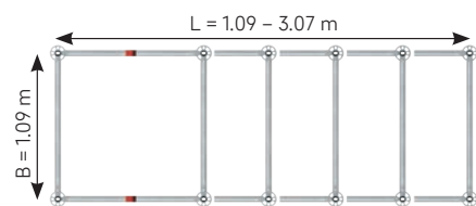
Bay length adaptation with Allround serial ledgers from 1.09 m to 3.07 m.
