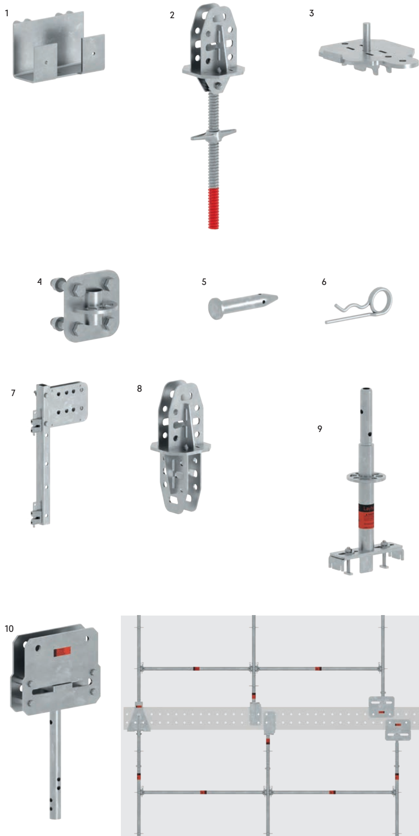
Suspended beams
