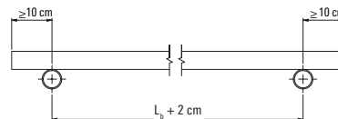
punctual bearing
