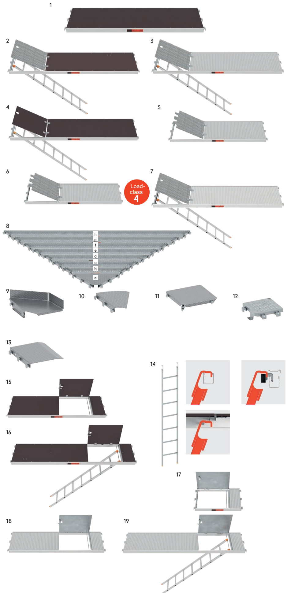
Installation situation 90° 9
