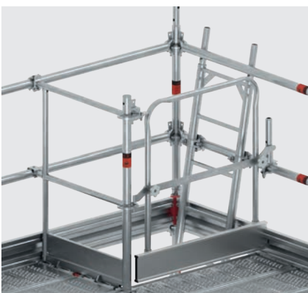
Installation situation of Allround O-side part 13
