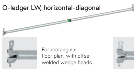
Distinction between right and left horizontal diagonal brace
